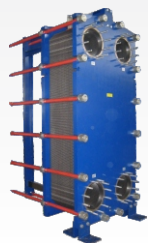
Plate Heat Exchanger
