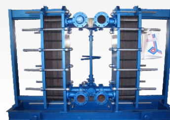
Double Module Plate Heat Exchanger
